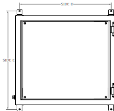
FRONT VIEW W/O COVER
