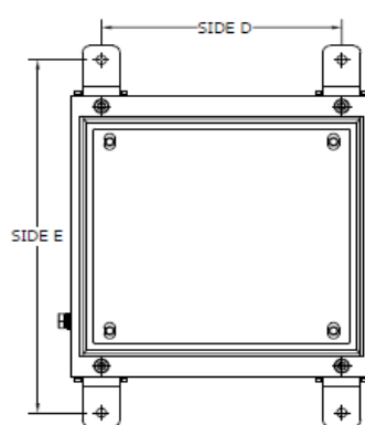
FRONT VIEW W/O COVER
